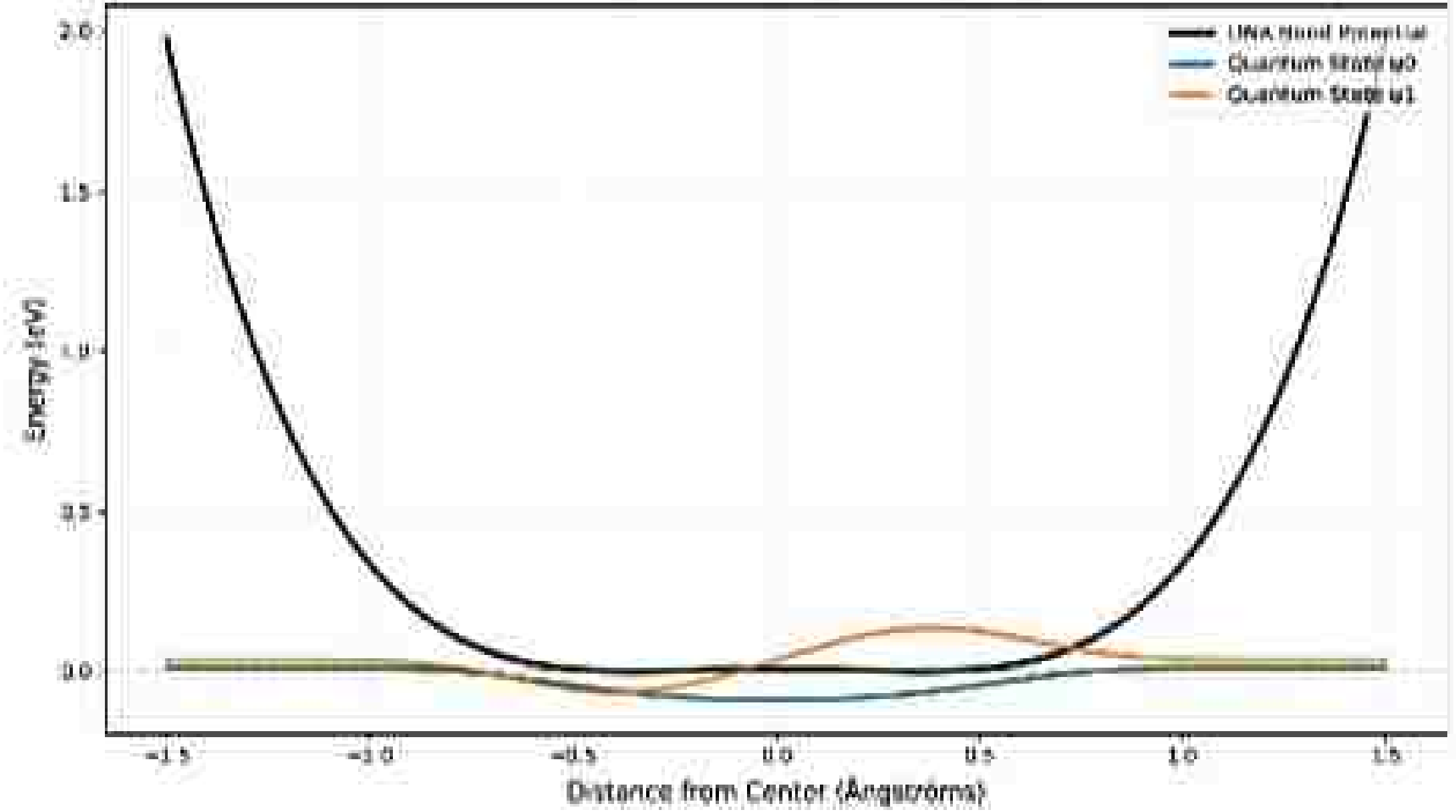
Proton Tunneling in Guanine-Cytosine Hydrogen Bond
