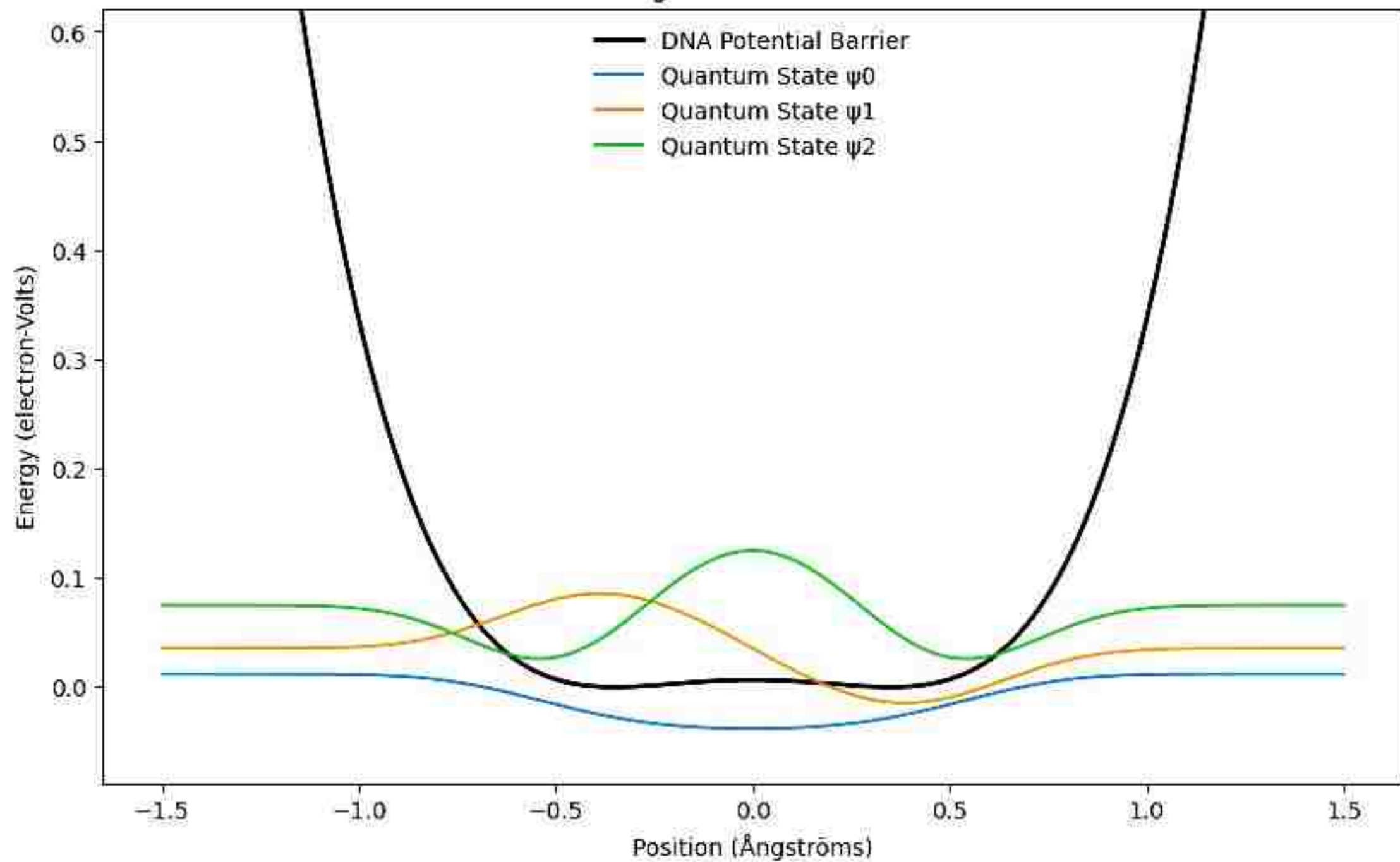
Proton Tunneling Simulation in DNA Base Pair
